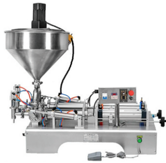
Double Head Paste Filling Machine
